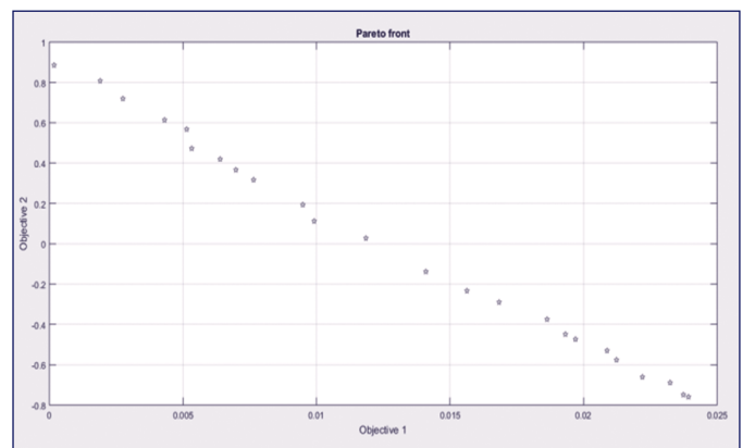
Fig.10 Pareto Front of Response (MRR &amp; Taper Angle)
