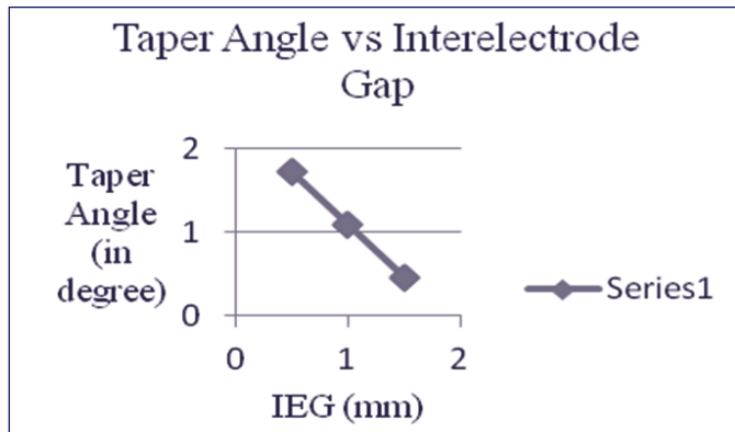
Fig.7 Taper angle v/s Inter electrode gap
