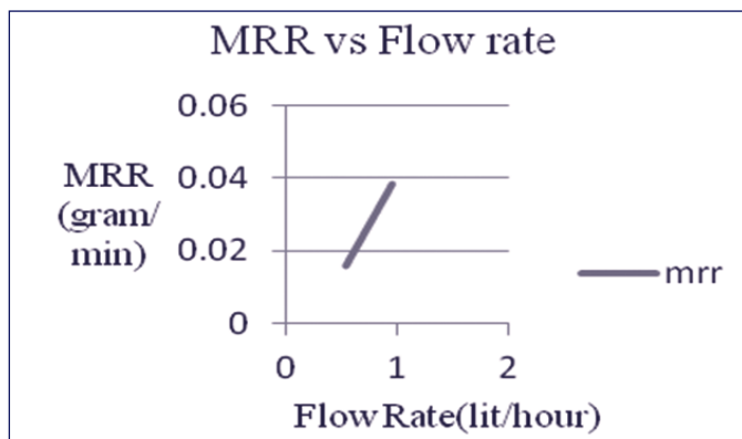
Fig.8 Graph of MRR v/s Flow Rate
