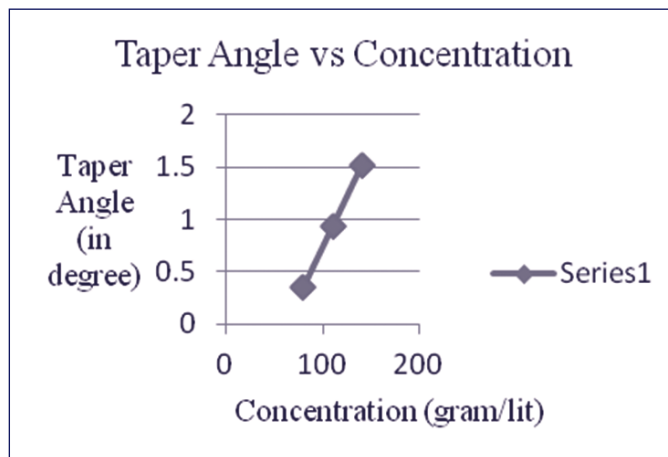
Fig.5 Graph of Taper angle v/s Concentration
