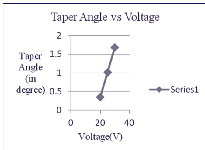
Fig.3 Graph of Taper angle v/s Voltage
